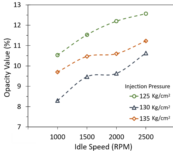
Figure 4. The comparison of opacity value and engine speed
