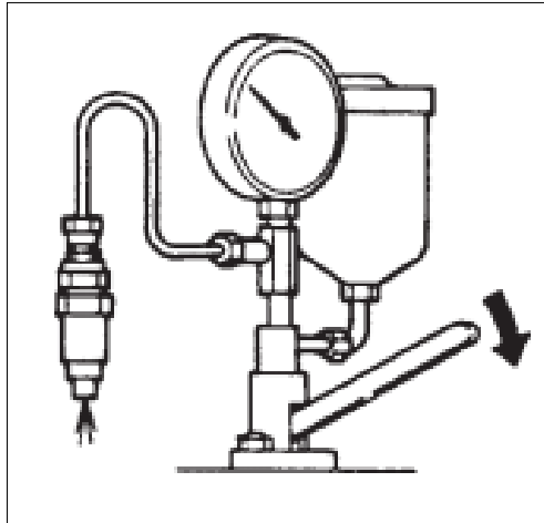
Figure 2. Nozzle tester
